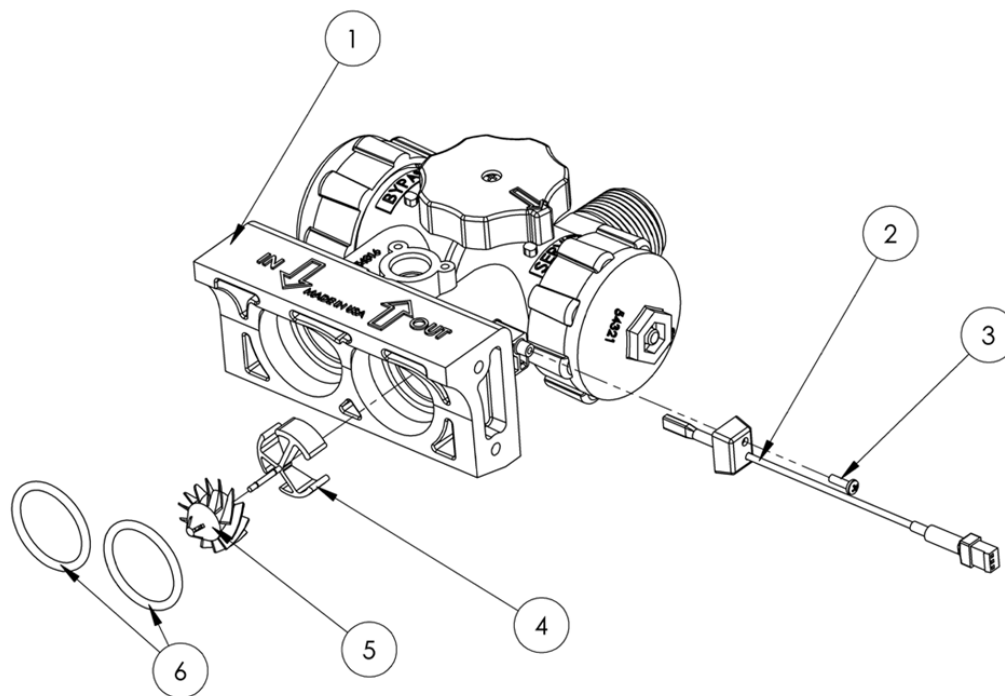
Figure 16: Bypass Assembly
