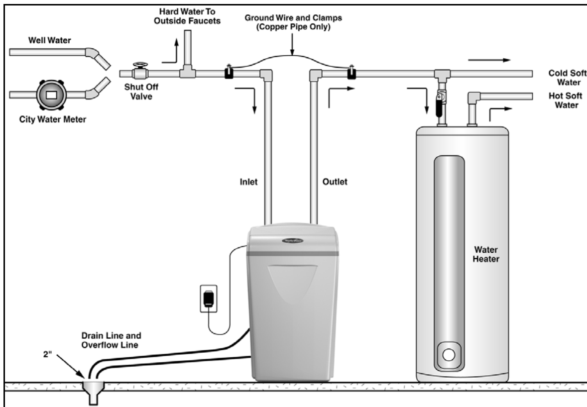
Figure 1: Appliance Placement
